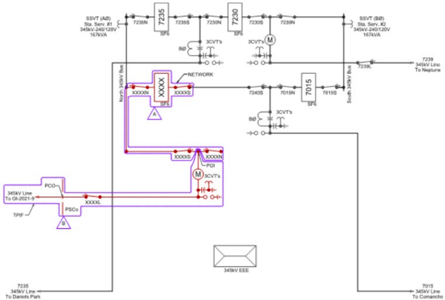
Figure 6 – Preliminary One-line of the GI-2021-9 POI at the Tundra 345 kV Substation
